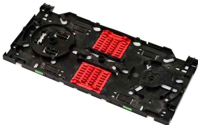
Cassette with an option for 24 fusion splices
